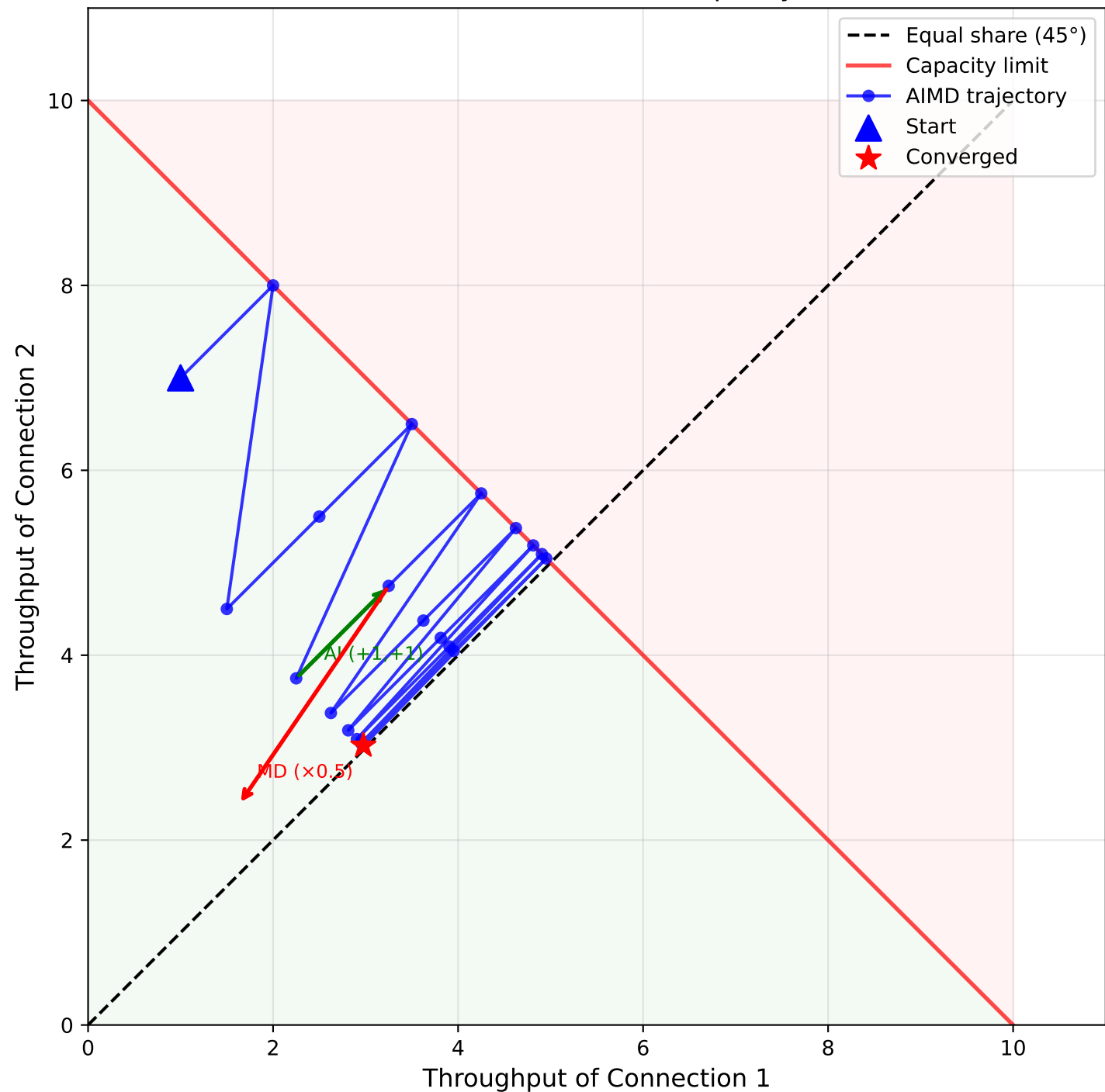
AIMD Fairness Convergence (Two TCP Connections, Link Capacity R=10)
